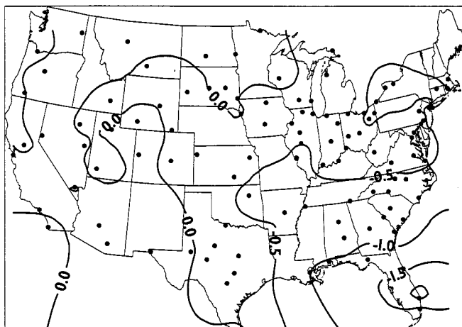
Figure 6. Dew point change for winter DP air mass ( ^{\circ}\text{C}/\text{decade} ). Dots represent stations used in winter analyses (this map only)
