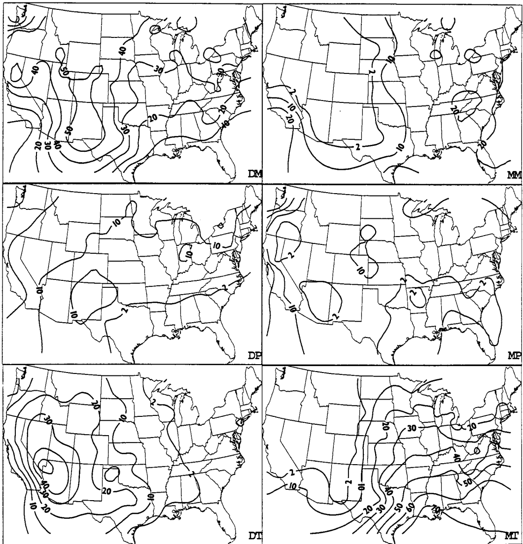
Figure 1. Mean air mass frequency for summer
