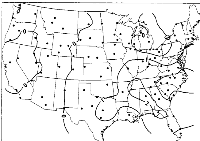
Figure 4. Frequency change for summer MT air mass (%/decade). Dots represent stations used in summer analyses (this map only)
