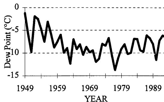
Figure 7. Mean annual dew point for the DP air mass, Atlanta, Georgia
