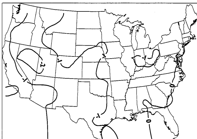
Figure 3. Frequency change for winter TR air mass (%/decade)
