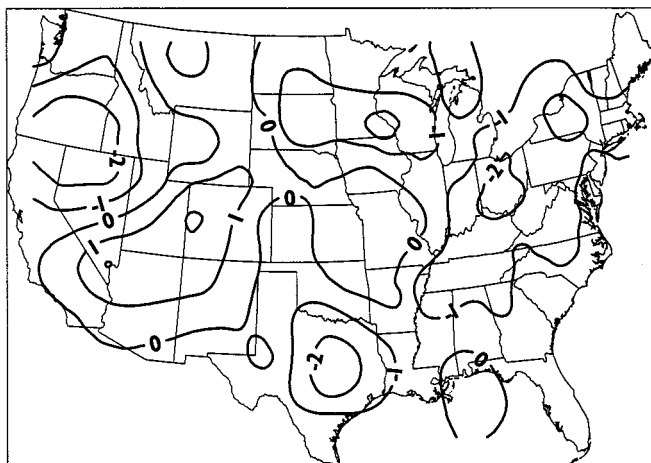
Figure 5. Frequency change for summer DM air mass (%/decade)
