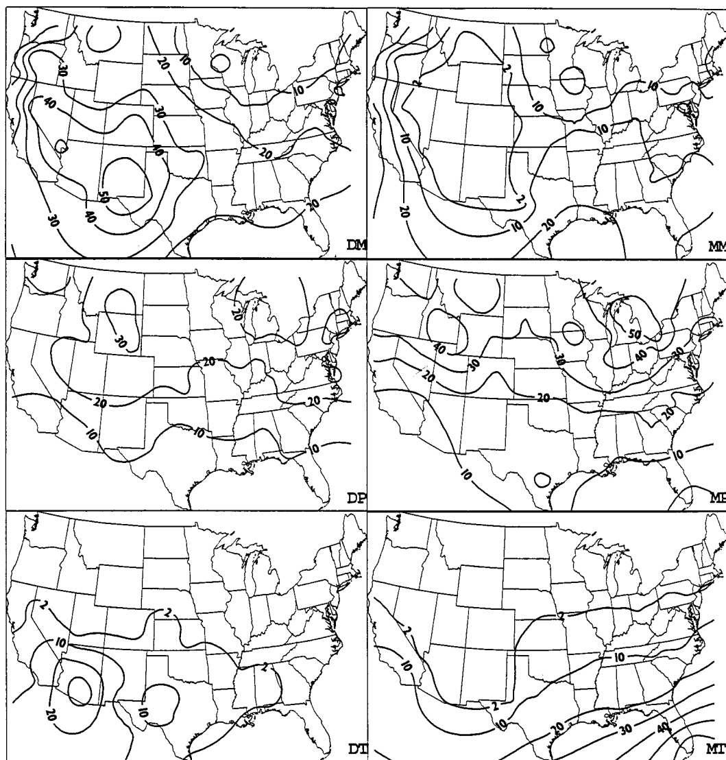
Figure 2. Mean air mass frequency for winter
